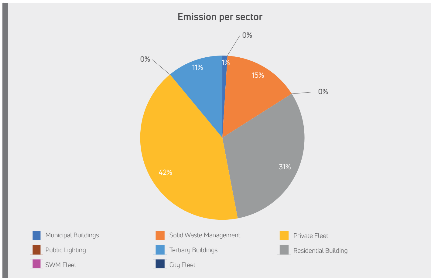
Figure 1: Emissions’ breakdown by sector
